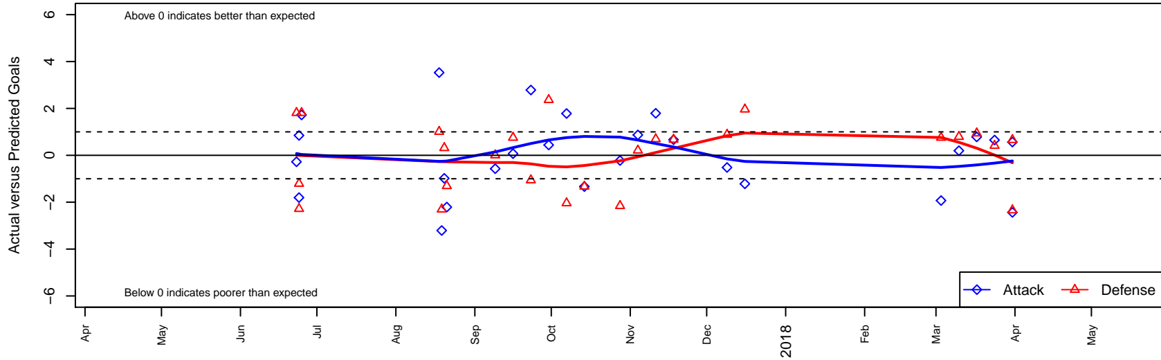
PSA Force Black B05 Dots are actual minus expected GF (blue circles) and GA (red triangles). Blue line is smoothed change in attack strength. Red is smoothed change in defense strength.
